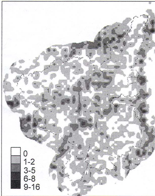
Fig. 1. Ignition density as number of ignitions in 25 years (1970–1994) in the Selway-Bitterroot Wilderness, Idaho and Montana.
