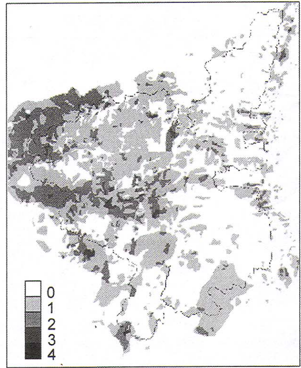
Fig. 4. Observed number of times burned in 115 years (1880-1994) in the Selway-Bitterroot Wilderness, Idaho and Montana.
