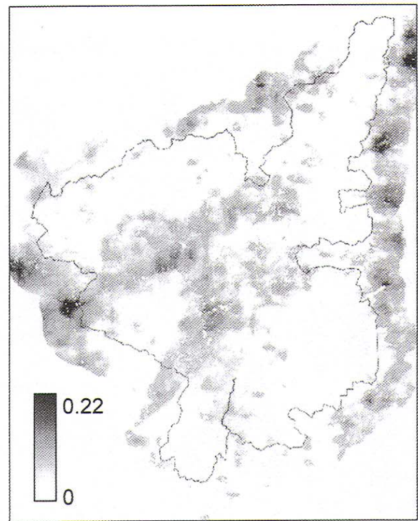
Fig. 2. Annual probability of burning predicted by mechanistic modeling approach in the Selway-Bitterroot Wilderness, Idaho and Montana.
