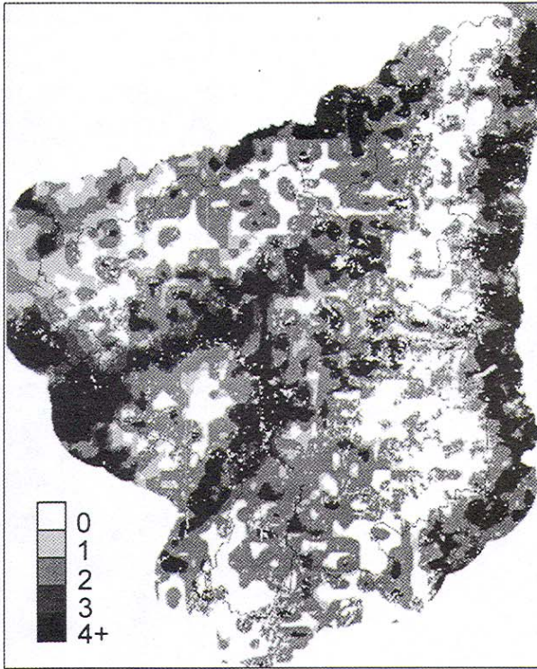
Fig. 3. Predicted number of times burned in 115 years in the Selway-Bitterroot Wilderness, Idaho and Montana.
